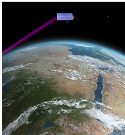
An instrument on Sentinel-6B will track radio signals from orbiting navigation satellites to measure physical properties of Earth's atmosphere. Credit: NASA-JPL/Caltech
